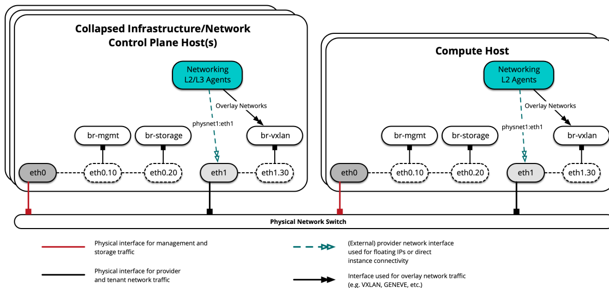
Network Interface Layout - Multiple Interfaces
