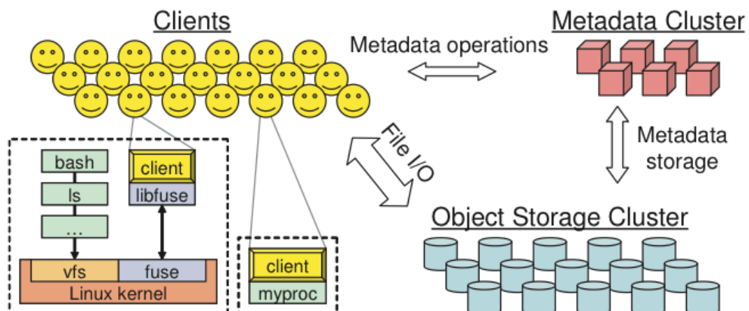
Fig. 1: Ceph architecture
